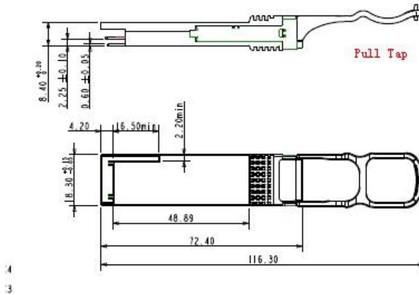
Figure 9. Mechanical Specifications
