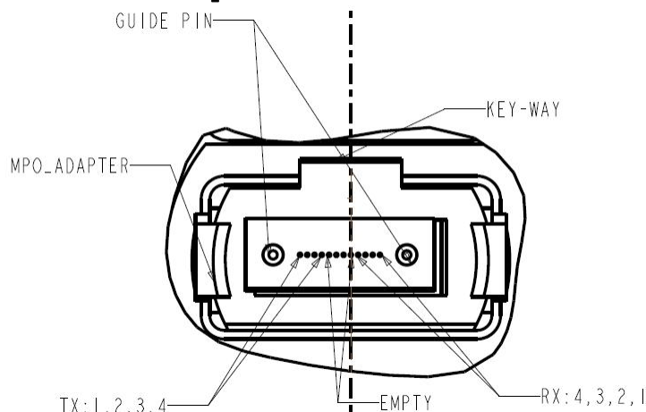
Figure 4. 40G QSFP+ PSM LR4 10km Optical Interface
