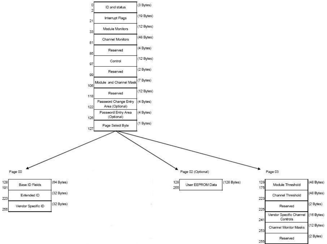
Figure5. QSFPE Memory Map
