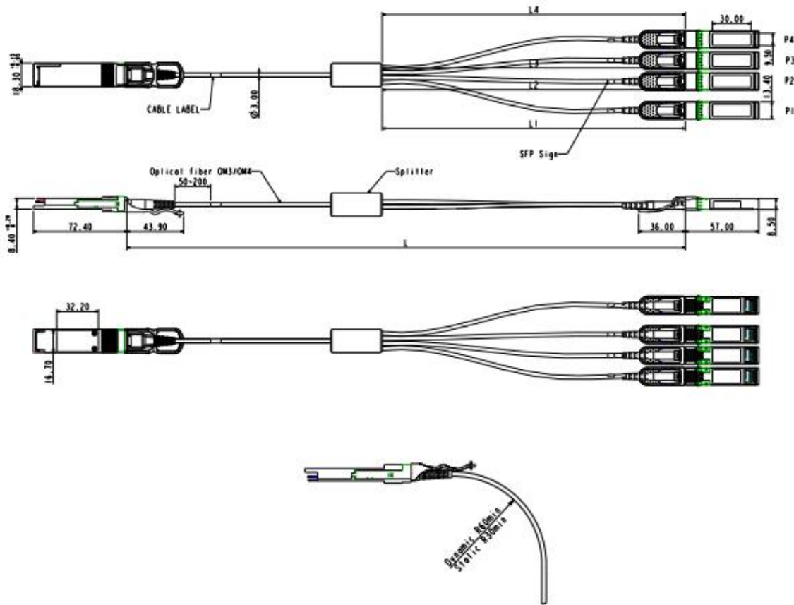
Figure1. Mechanical Specifications
