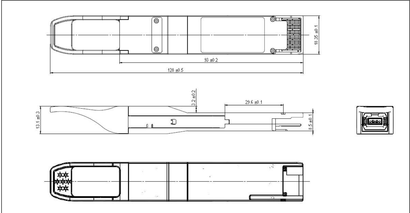
Figure10. Mechanical Specifications
